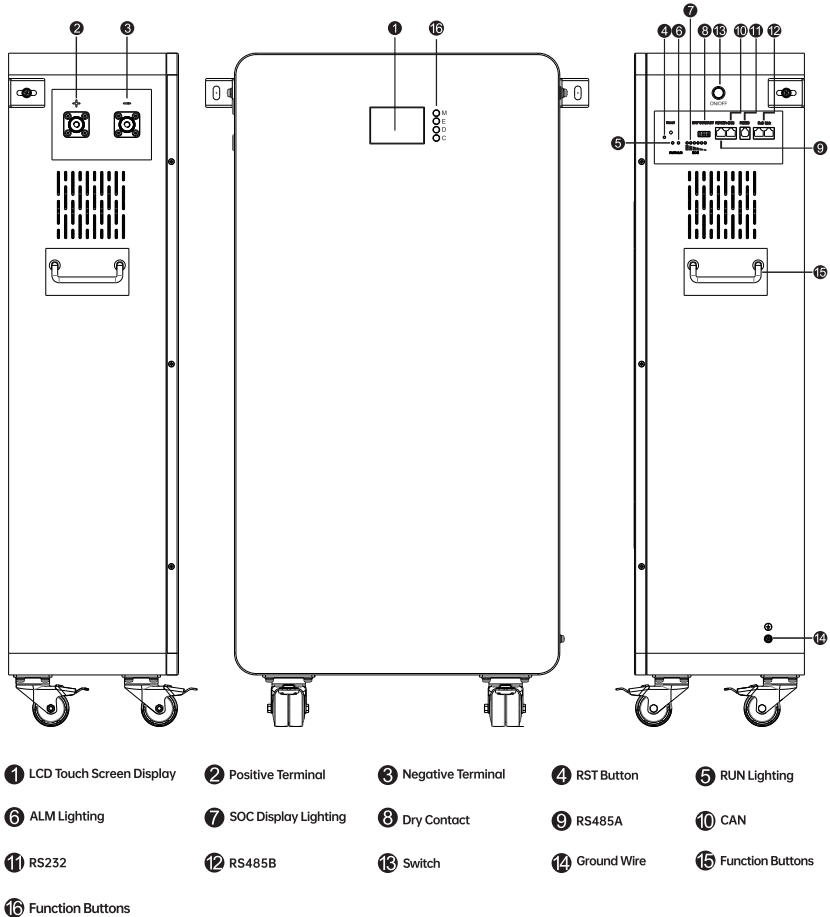
Figure 2 Control Panel Illustration (Reference Picture)
